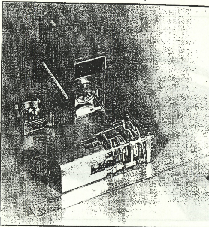
Figure 7. MC2969 Intent Stronglink Switch
